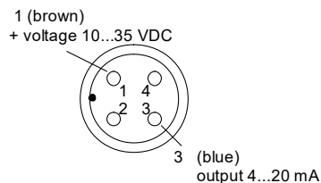
M12 plug with PMU
