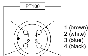
M12 plug (only PT100)
