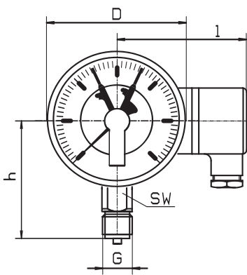
Connection bottom
