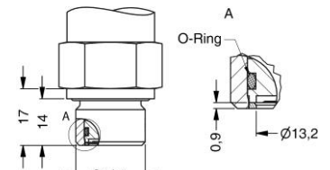
G1/2" DIN 3852 with flush sensor
